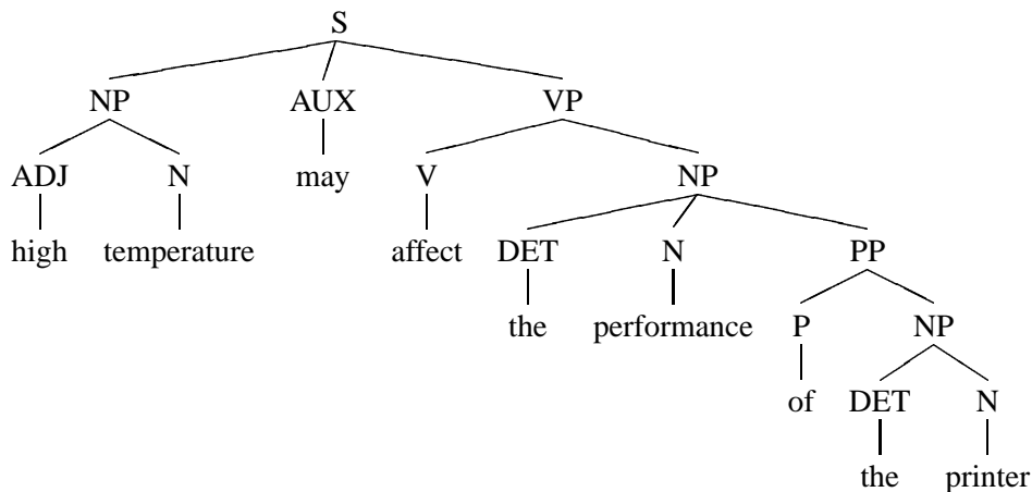
Figure 3.3 A More Complex Tree Structure
